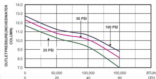
FLOW CHARACTERISTIC CHART FOR MODEL GR-700
